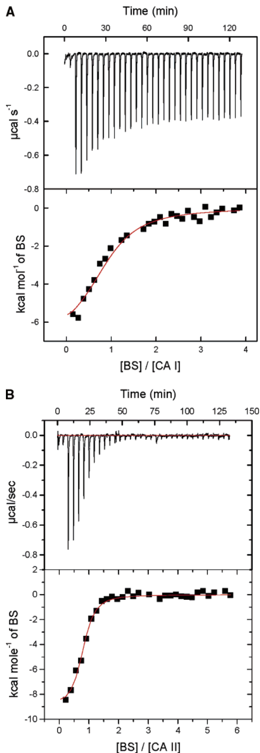
Figure 1. Isothermal microcalorimetric titration data for the binding of benzenesulfonamide (BS) to recombinant human carbonic anhydrase isozymes I (A) and II (B). The upper and lower panels represent the raw calorimetric data and fitted data, respectively. The solid smooth lines represent the best fit of the data for the binding of benzenesulfonamide to CA I (A) with stoichiometry n = 0.9 , association constant K_a = 3.8 \times 10^5 \text{ M}^{-1} , and \Delta H^\circ = -7.1 \text{ kcal/mol} . The corresponding parameters for the binding of benzenesulfonamide to CA II are 0.8, 1.7 \times 10^6 \text{ M}^{-1} , and -9.1 \text{ kcal/mol} , respectively.
