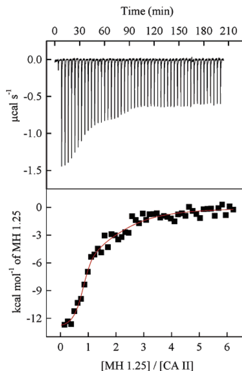
Figure 2. Isothermal microcalorimetric data for the binding of MH 1.25 to CA II. Note the raw data (top panel) shows two inflection points, consistent with two-site binding. The solid smooth line is the best fit of the data according to the two binding site model for the following stoichiometries ( n_1, n_2 ), association constants ( K_{a1}, K_{a2} ), and enthalpic changes ( \Delta H^\circ_1, \Delta H^\circ_2 ); 0.8, 1.5, 1.0 \times 10^7 \text{ M}^{-1} , 2.1 \times 10^5 \text{ M}^{-1} , -13.0 \text{ kcal mol}^{-1} , and -6.1 \text{ kcal mol}^{-1} , respectively.
